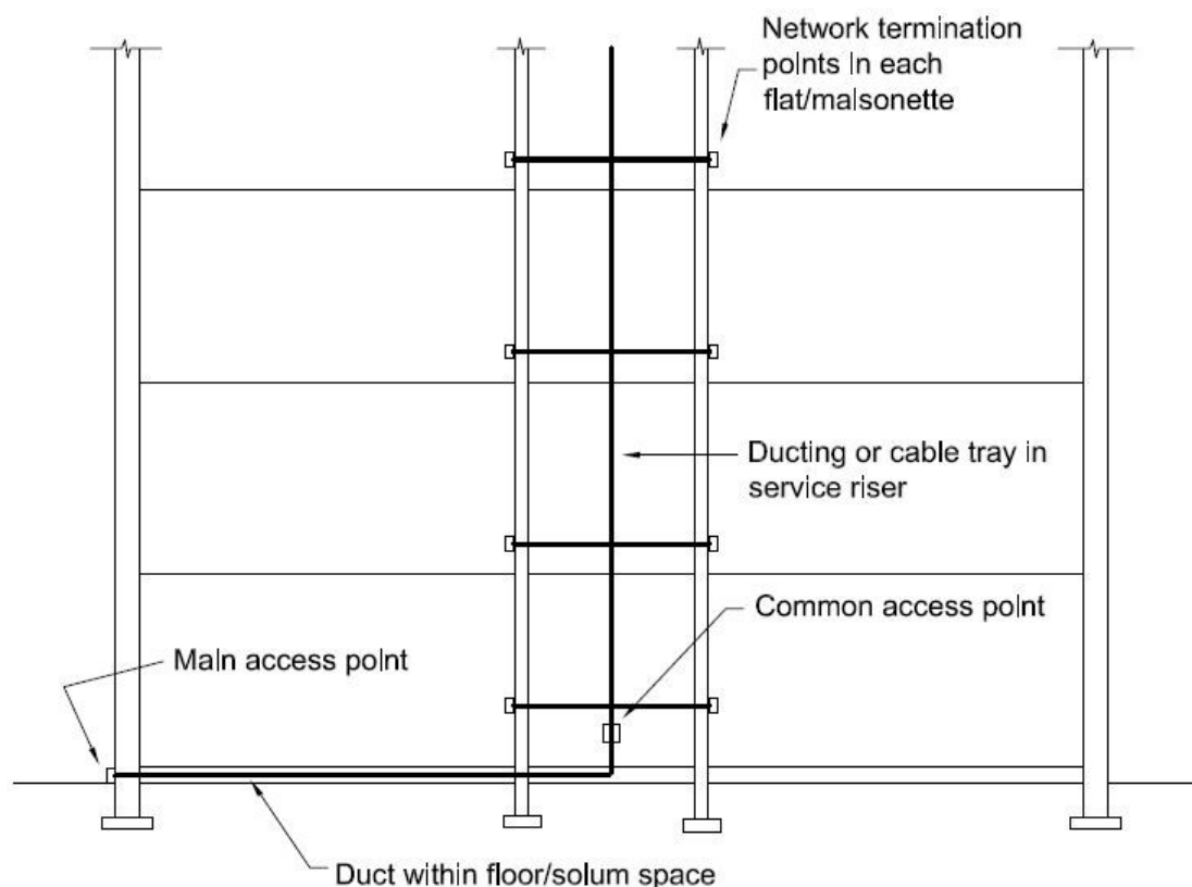
Figure 4.16 Typical in-building infrastructure for flats and maisonnettes
