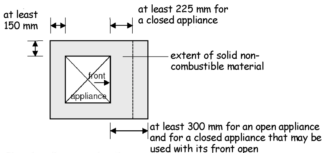
Plan of appliance on a hearth
