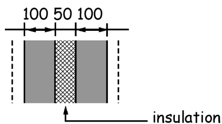
Figure 3.15 Wall constructions - Type C
