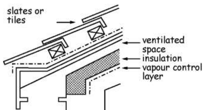
Figure 3.35 Roof type B insulation on a sloping ceiling
