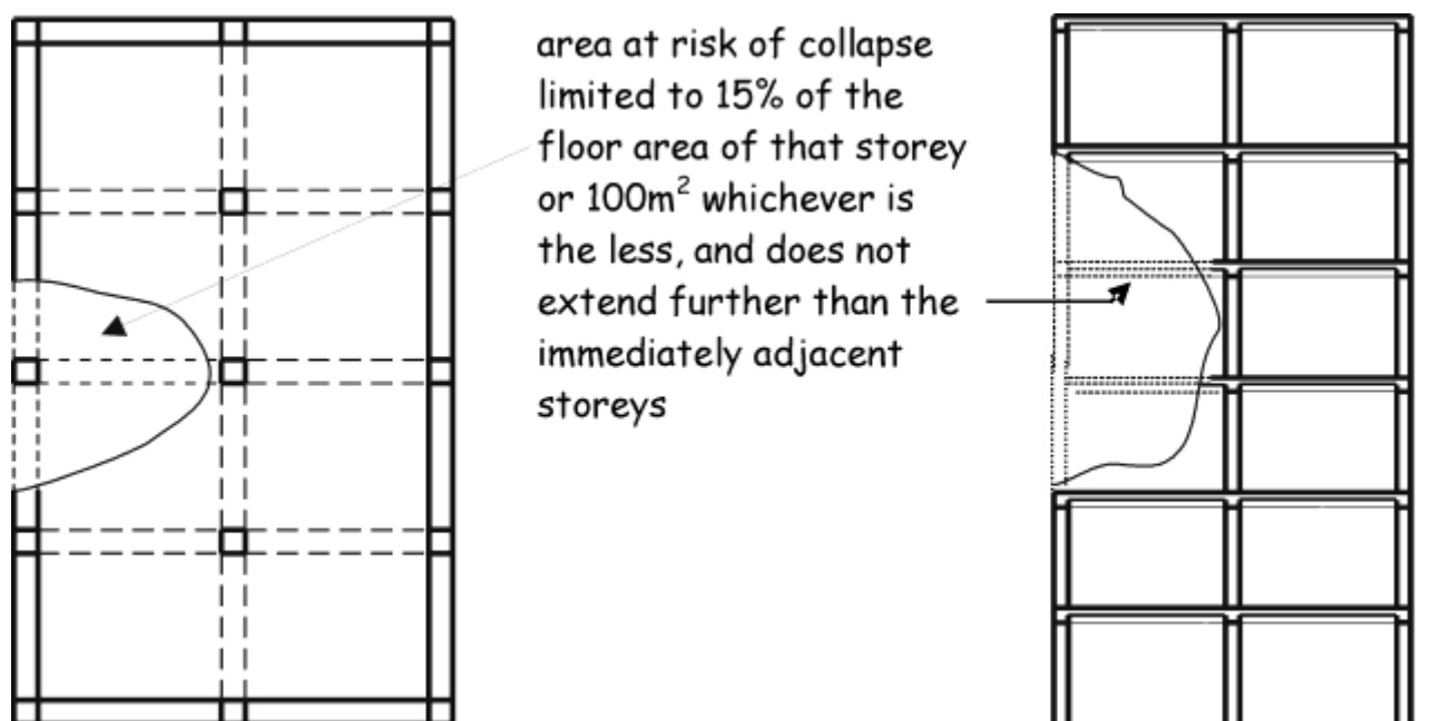
Figure 1.1 Floor collapse limit
