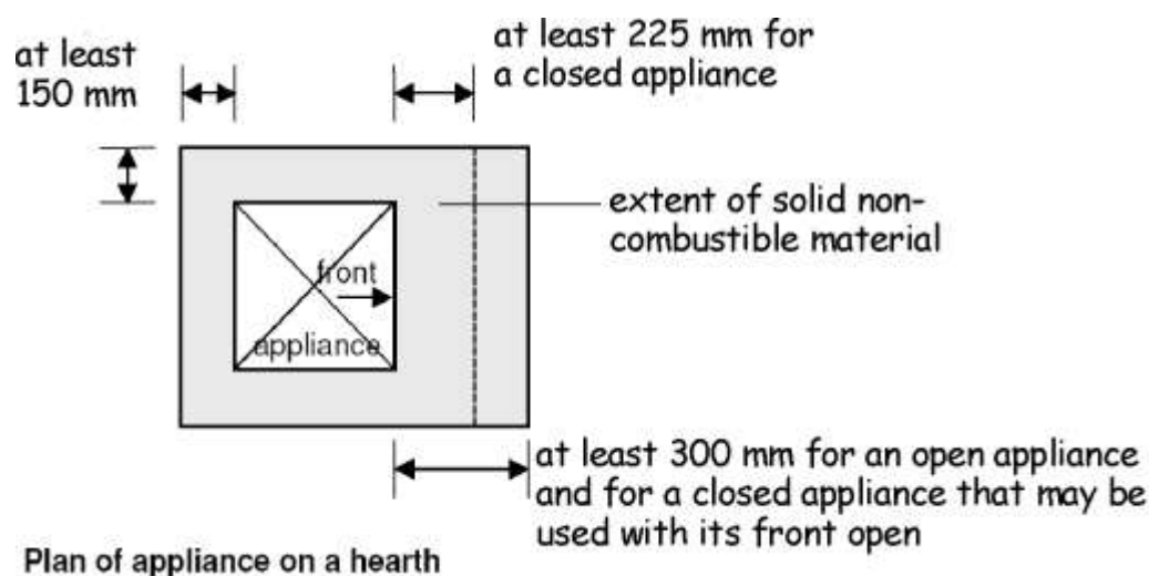
Figure 3.44 Appliance location
