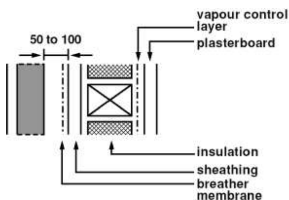
Figure 3.16 Wall constructions - Type A
