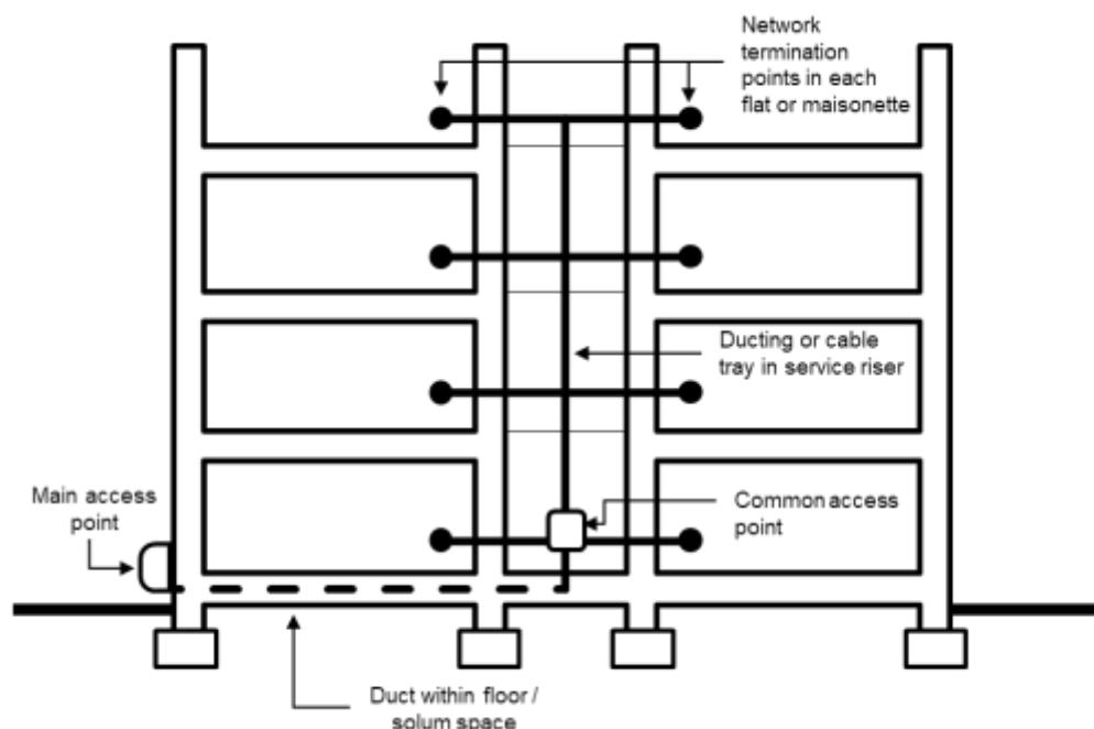
Figure 4.16 In-building infrastructure serving flats or maisonettes
