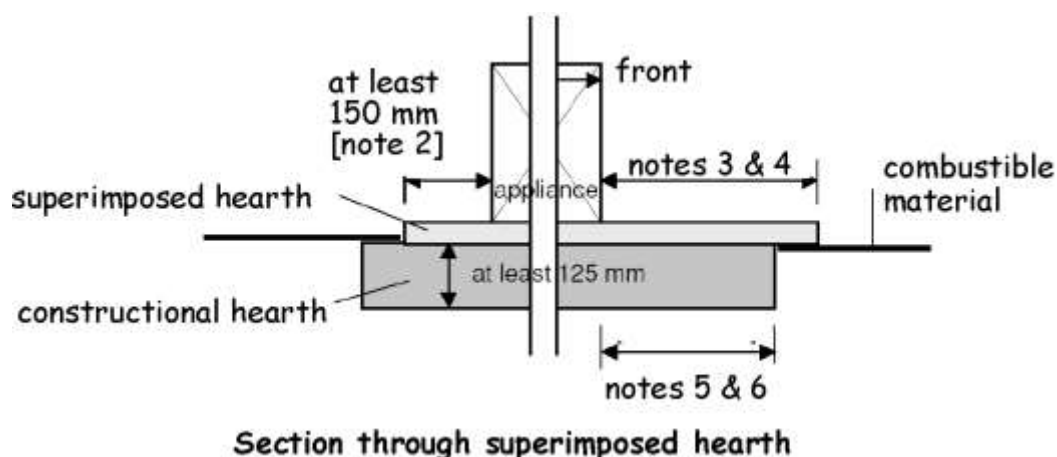
Figure 3.45 Superimposed hearths
