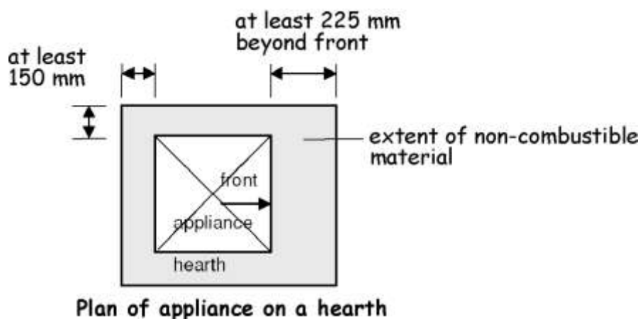
Figure 3.47 Plan of appliance on a hearth (gas-fired)
