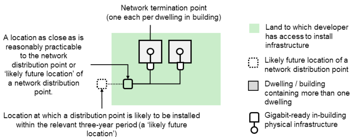
Figure 4.18 Onsite physical infrastructure to a location as close as reasonably practicable to a network distribution point or likely future location of a network distribution
