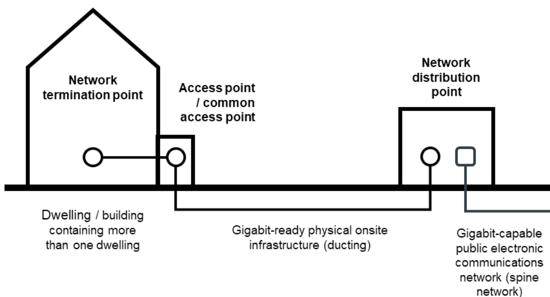
Figure 4.17 Wired connection – Onsite physical infrastructure linking to in-building physical infrastructure to a network distribution point
