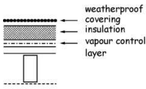
Figure 3.21 Roof constructions – Type C
