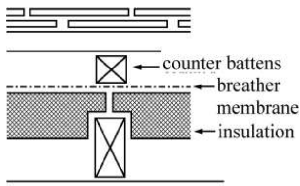
Figure 3.36 Roof type B insulation on a sloping ceiling
