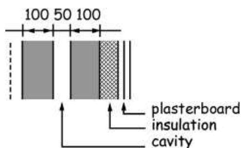
Figure 3.14 Wall constructions - Type B
