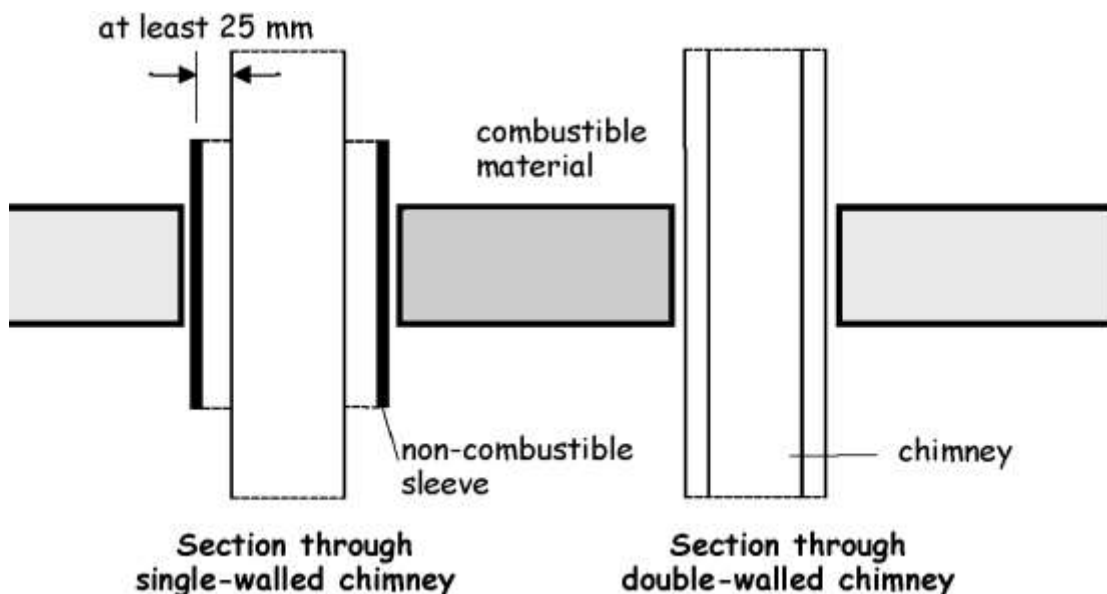
Figure 3.40 Section through single-walled Chimney (vertical)
