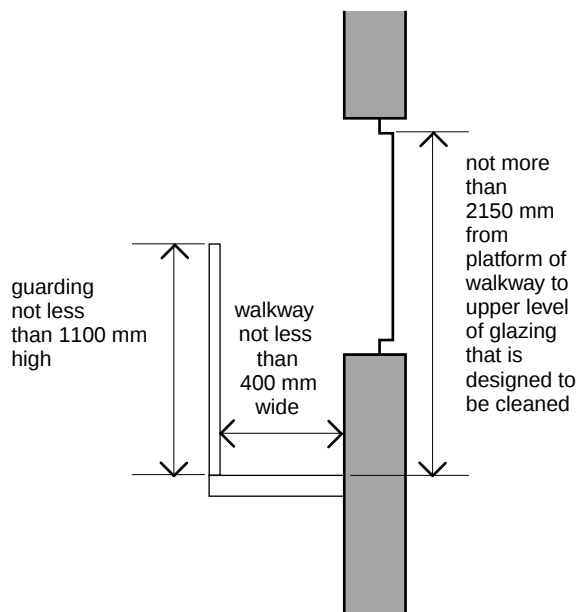
(b) walkway with guarding
