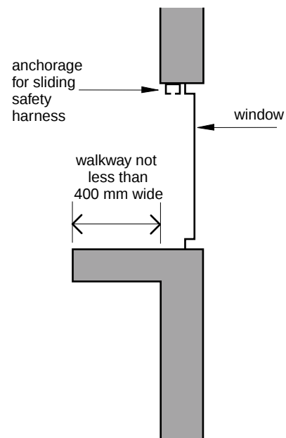
(c) walkway with anchorage for sliding safety harness
