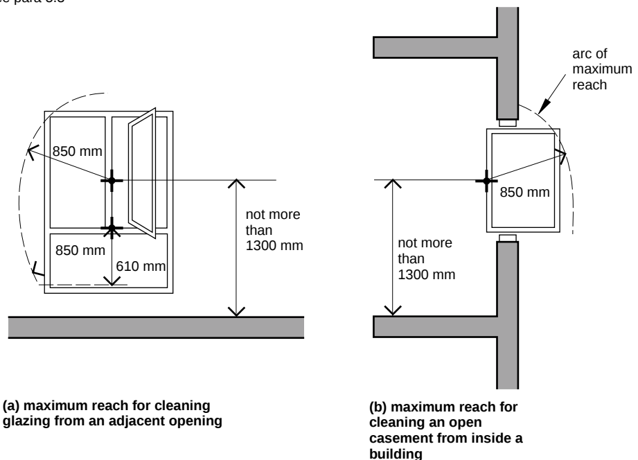
Diagram 5.1 Cleaning the external face of glazing from the inside
