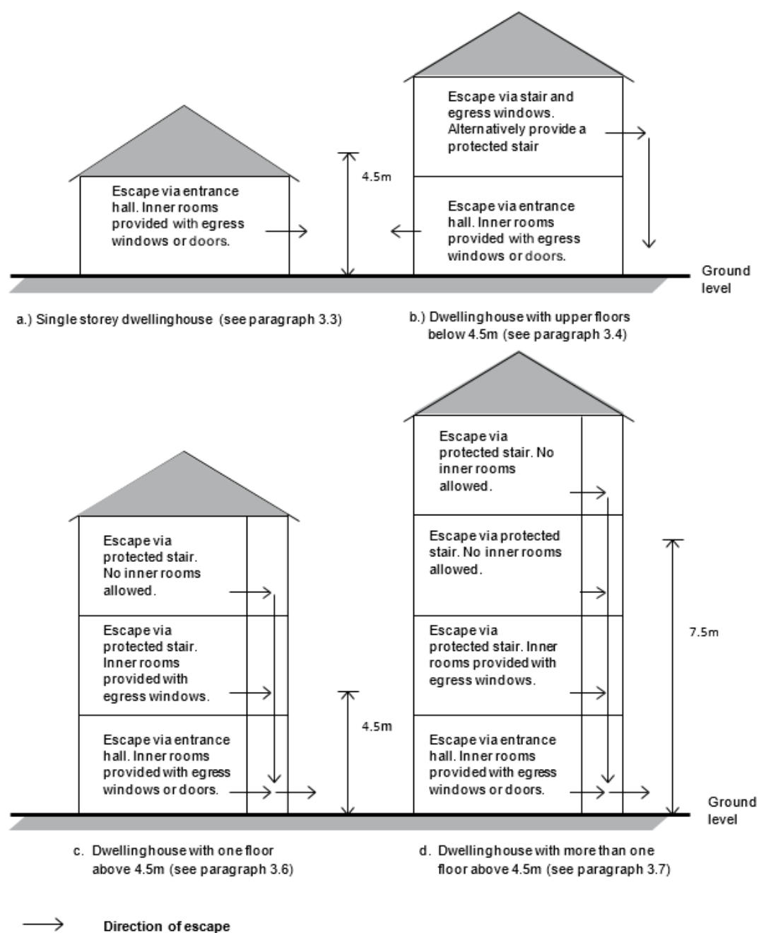
Diagram 1 Means of escape from dwellinghouses
