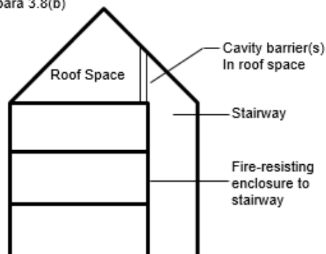
a. With cavity barriers
