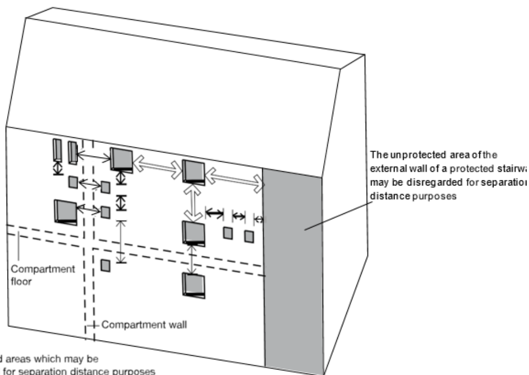
Diagram 20 Unprotected areas which may be disregarded in assessing the separation distance from the boundary
