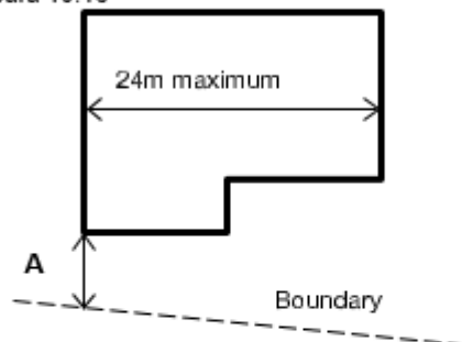
Diagram 22 Permitted unprotected areas for Method 1
