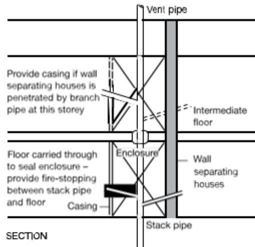
Diagram 15 Enclosure for drainage or water supply pipes
