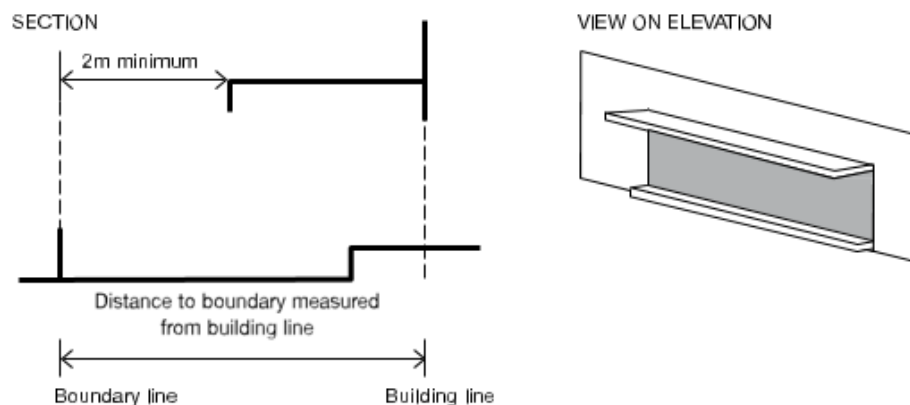
Diagram 21 The effect of a canopy on separation distance
