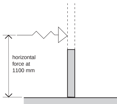
Diagram 5.1 Guarding
