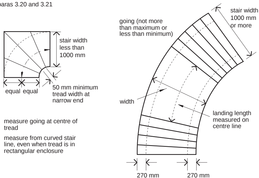
Diagram 3.7 Measuring tapered treads
