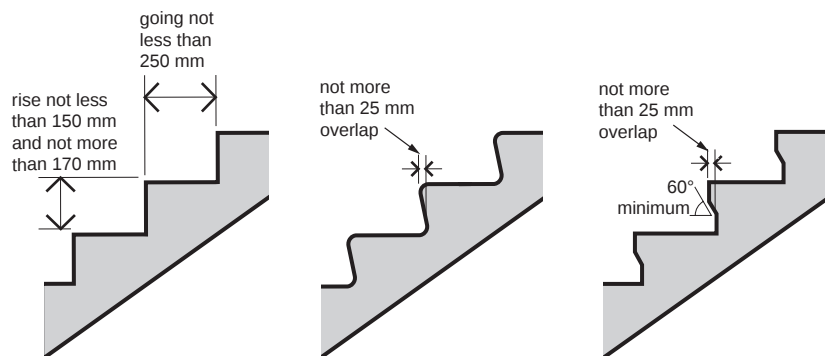
(b) examples of suitable step profiles
