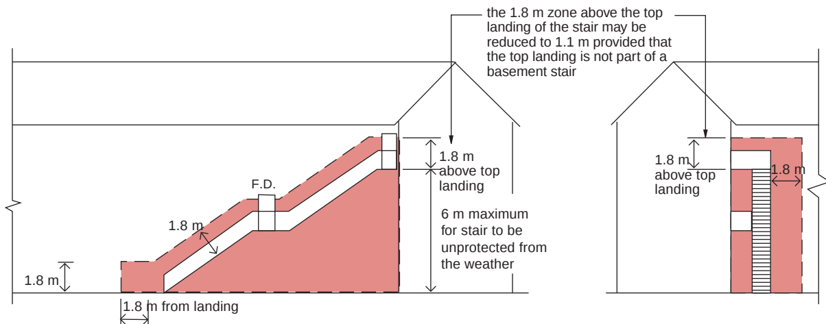
elevation b1
