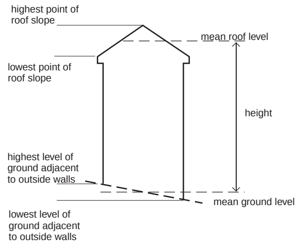
(a) Double pitch roof
