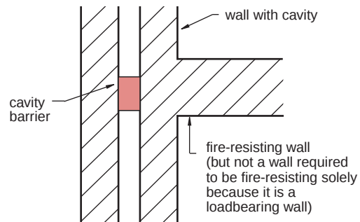
(c) Plan
