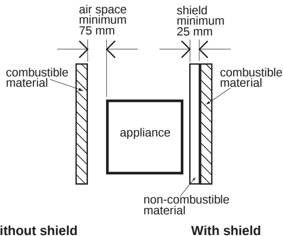
Diagram 4.8 Shielding of appliances
