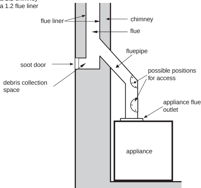
Diagram 1.1 Chimneys and flues
