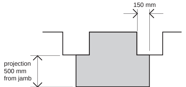
(a) Fireplace recess
