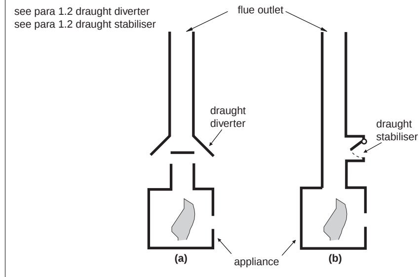
Diagram 1.2 Draught diverters and draught stabilisers
