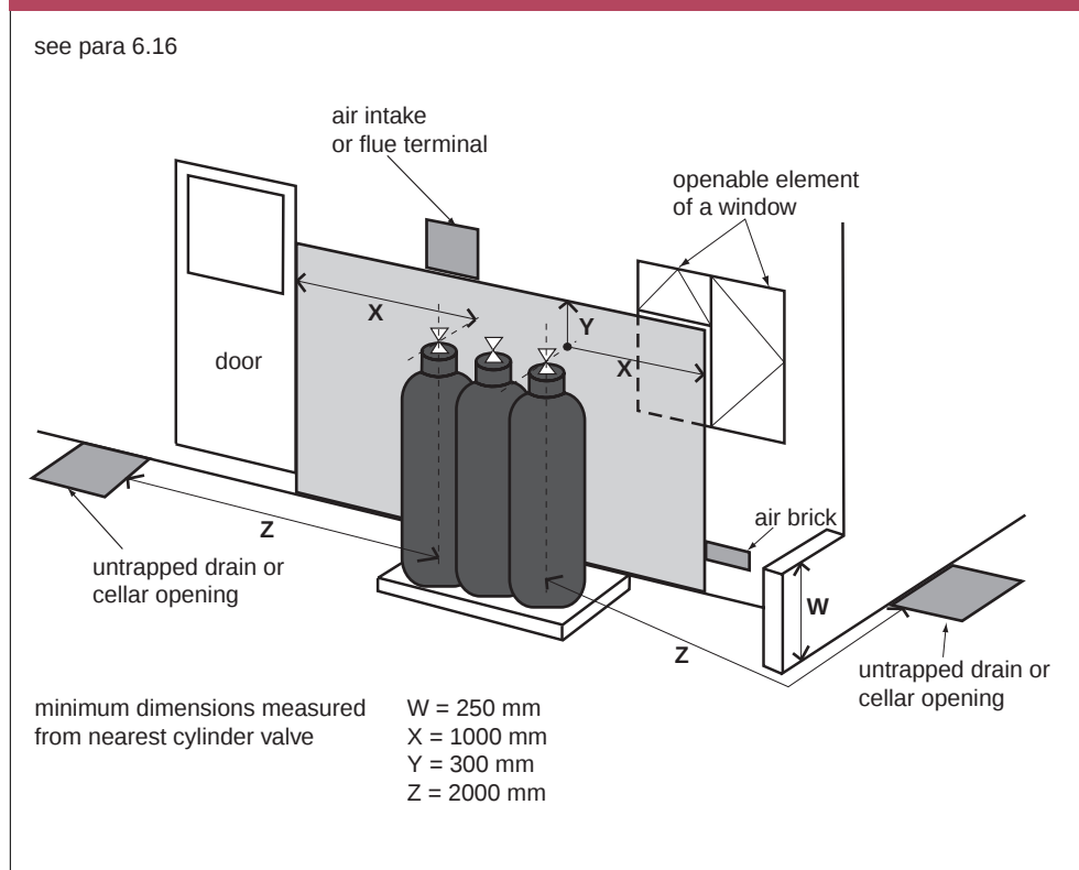
Diagram D1 Location of LPG cylinders
