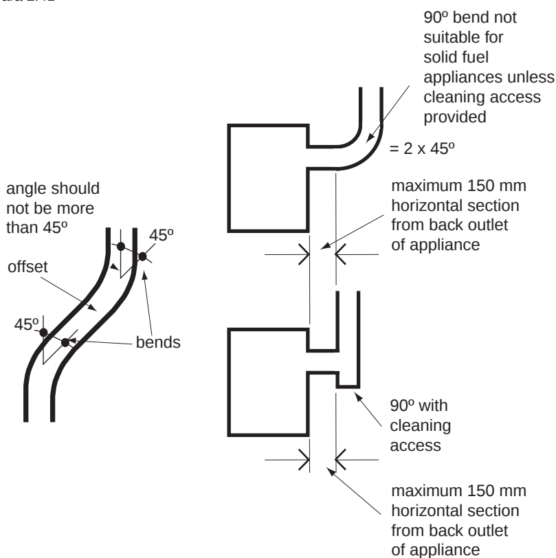
Diagram 2.7 Bends in flues
