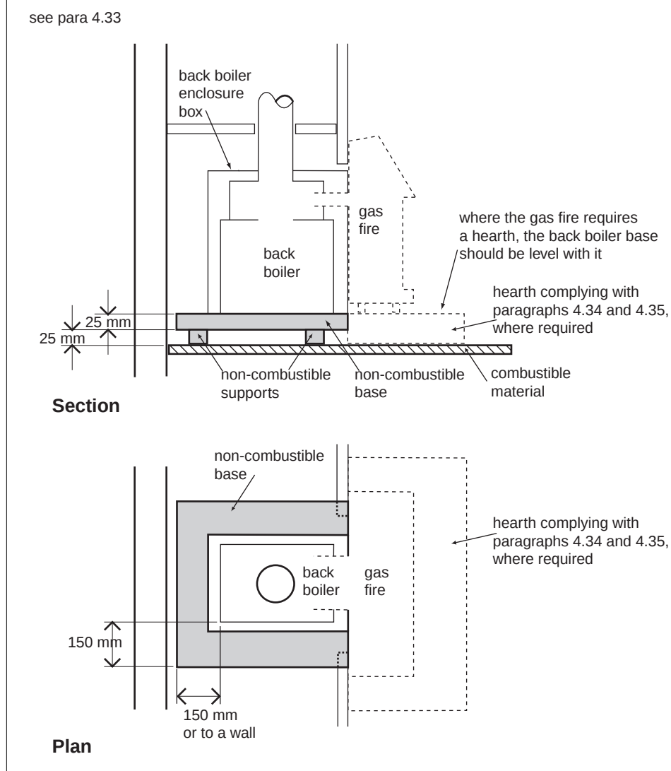
Diagram 4.5 Base for back boiler
