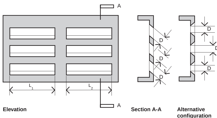
(a) Ventilator assembled on site from components
