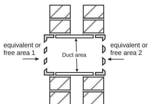
(a) Ventilator assembled on site from components
