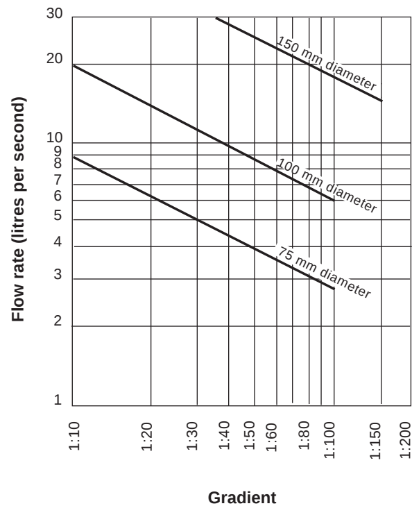
Diagram 4.1 Discharge capacities of rainwater drains running full
