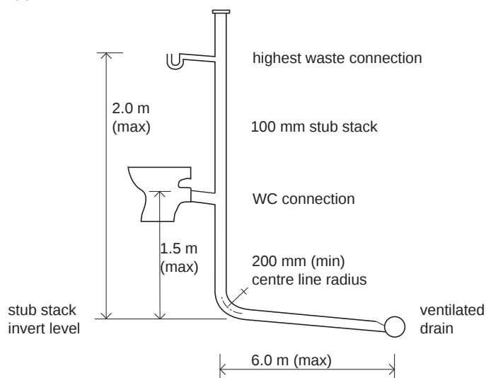
Diagram 2.6 Stub stacks
