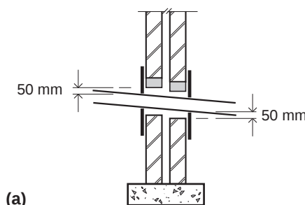
Diagram 3.6 Pipes penetrating walls
