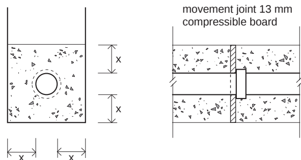
Diagram 3.4 Concrete encasement for rigid pipes
