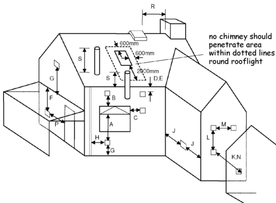
Figure 3.62 Gas-fired - flue outlets
