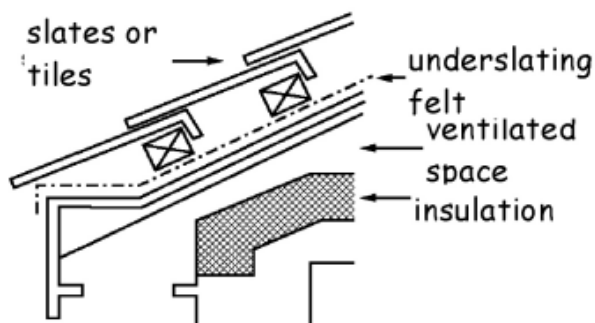
Figure 3.31 Roof constructions -Type A
