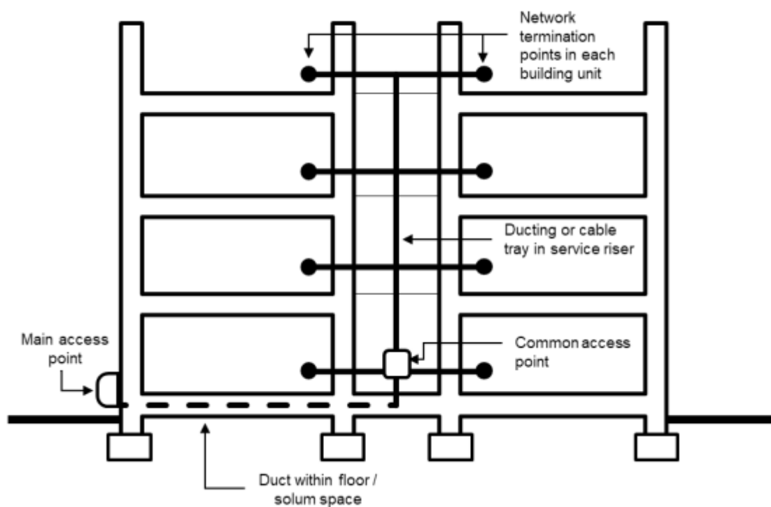
Figure 4.13 In-building physical infrastructure serving multi-occupancy buildings
