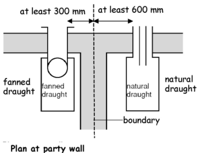
Figure 3.63 Separation between a boundary and terminal at right angles
