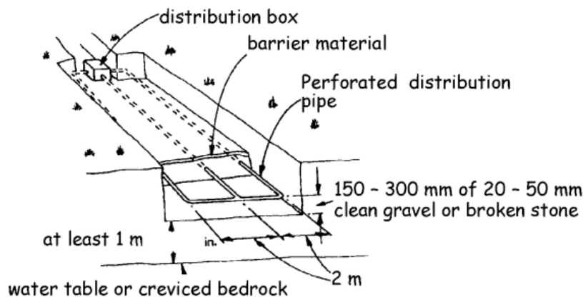
Figure 3.15 Piped infiltration bed system
