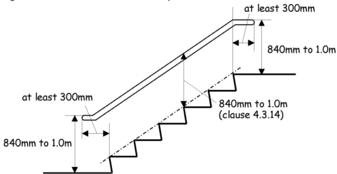
Figure 4.7 Handrails to stairs and ramps
