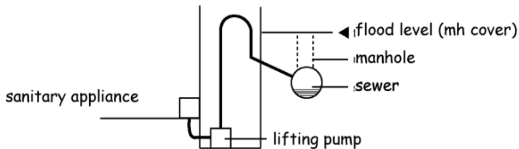
Figure 3.13 Diagrammatic section through a pumped system in a basement
