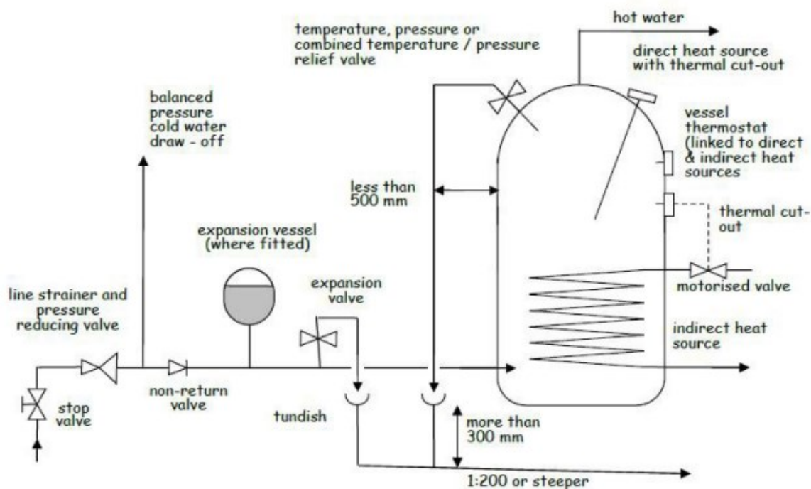
Figure 4.9 Unvented hot water storage system – indirect example
