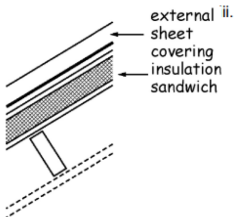
Figure 3.34 Roof constructions - Type D
