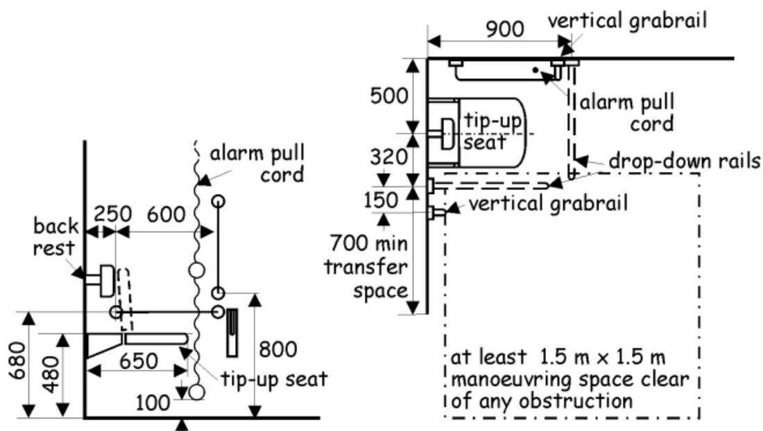
Figure 3.39 Provisions within an accessible changing facility
