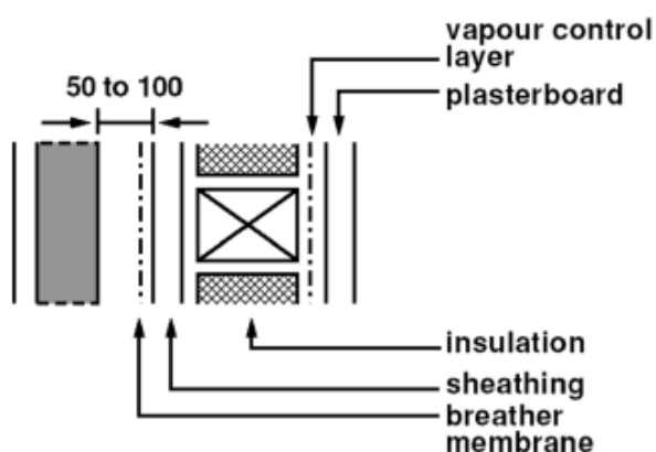
Figure 3.22 Wall constructions - Type A
