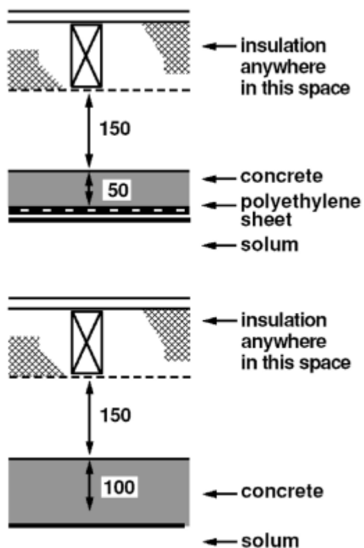
Figure 3.12 Suspended timber floors 2
