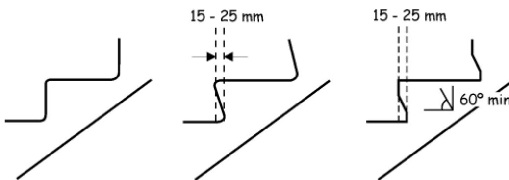
Figure 4.5 Step profile examples
