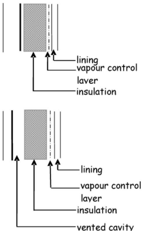
Figure 3.24 Wall constructions - Type C
