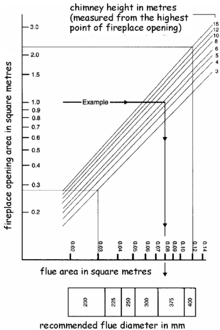
Figure 3.56 Flue sizing for larger solid fuel open fires
