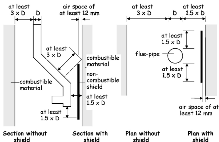
Figure 3.46 Relationship of flue-pipes to combustible material
