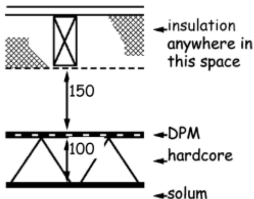
Figure 3.11 Suspended timber floors 1
