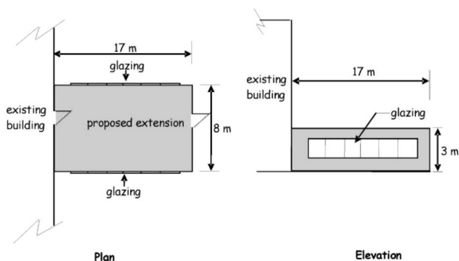
Figure 6.1. Extension example
