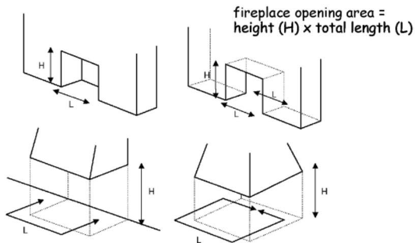
Figure 3.56 Flue sizing for larger solid fuel open fires
