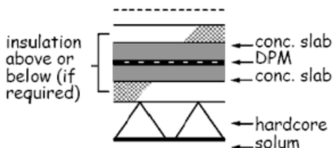
Figure 3.9 Ground supported concrete floors 3
