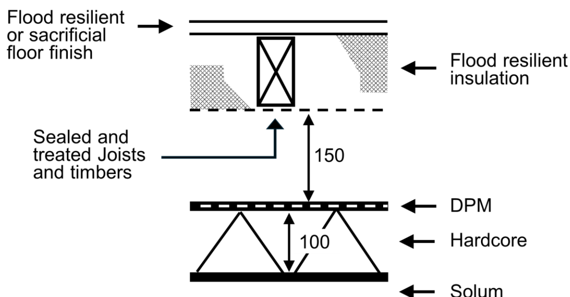
Figure 3.3 Suspended timber floor
