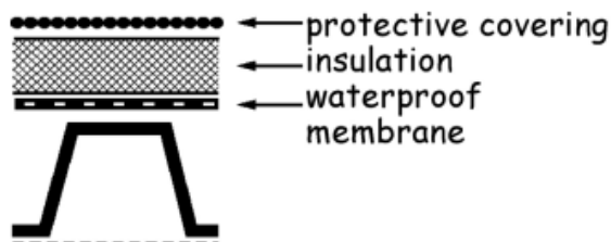
Figure 3.30 Roof constructions - Type F
