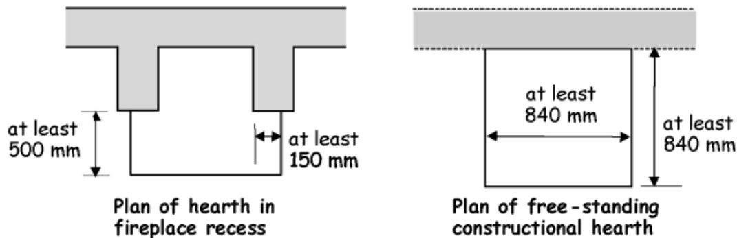
Figure 3.47 Hearth construction
