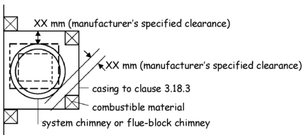
Figure 3.43 Plan of casing round a factory-made chimney
