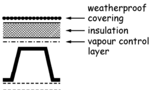
Figure 3.29 Roof constructions - Type E
