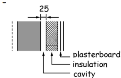
Figure 3.17 Wall constructions -Type A
