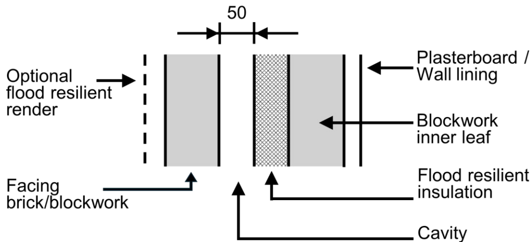
Figure 3.5 Wall construction – cavity wall with partial fill insulation
