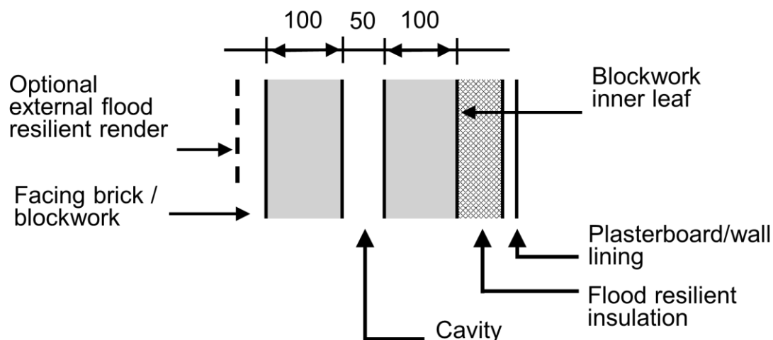
Figure 3.4 Wall construction – cavity wall with internal insulation
