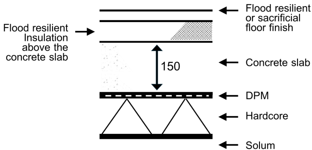
Figure 3.1 Ground supported concrete floor
