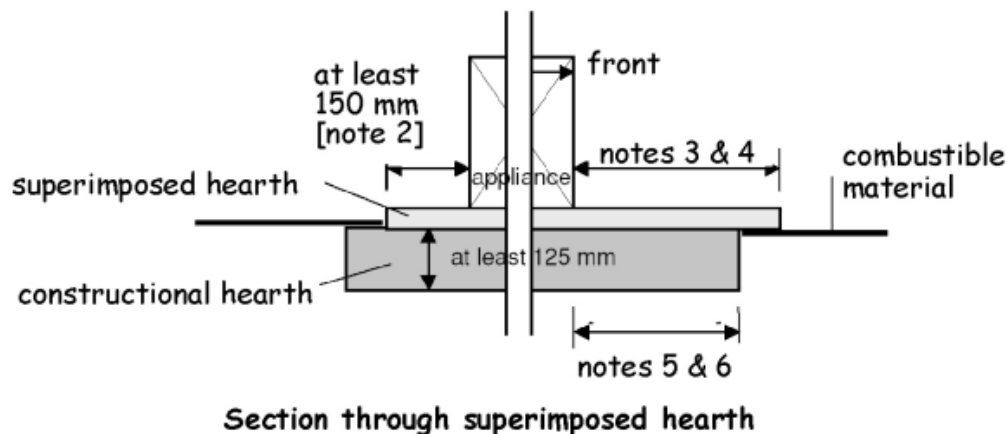
Figure 3.49 Superimposed hearths
