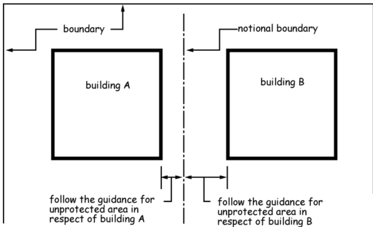
Figure 2.6 Notional Boundary
