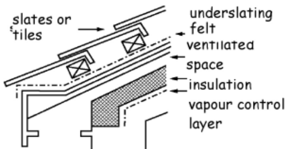
Figure 3.32 Roof constructions -Type B
