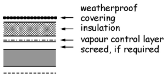
Figure 3.25 Roof constructions -Type A
