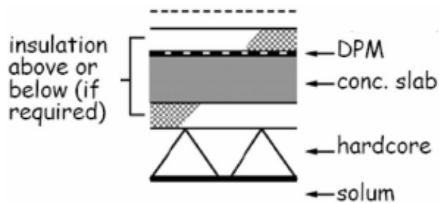
Figure 3.7 Ground supported concrete floors 1
