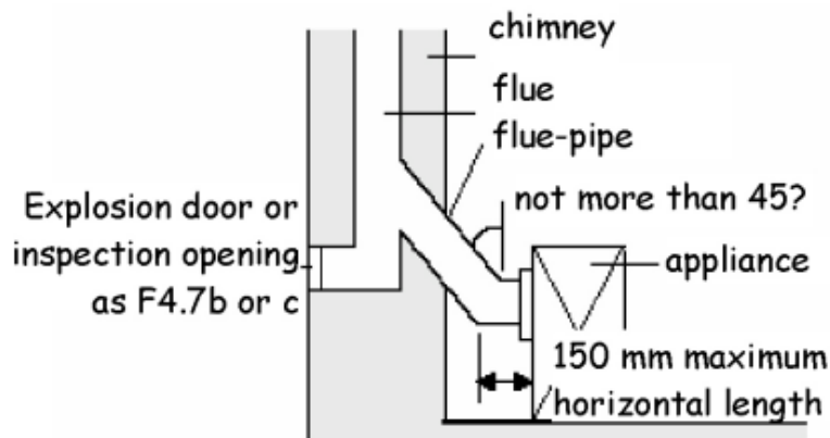
Section through appliance and flue-pipe
