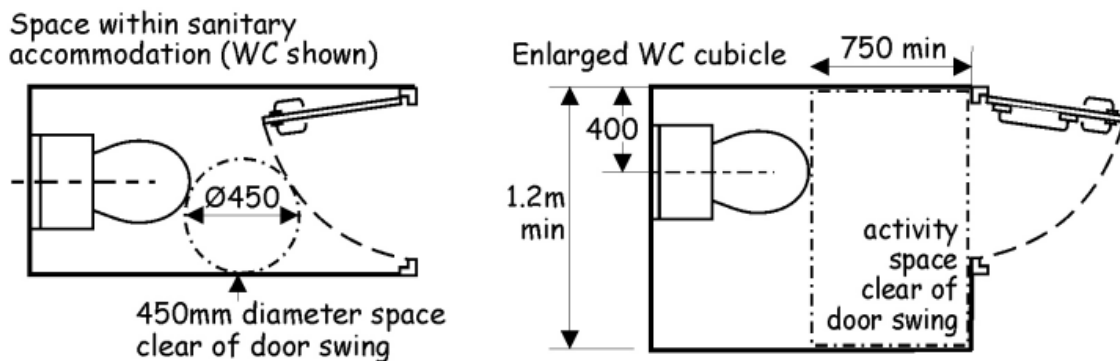
Figure 3.35 Space within sanitary accommodation and enlarged WC Cubicle
