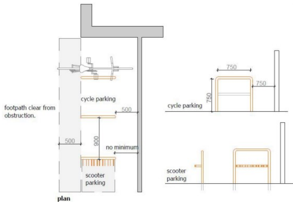
Figure 7.6 Example of cycle and scooter parking
