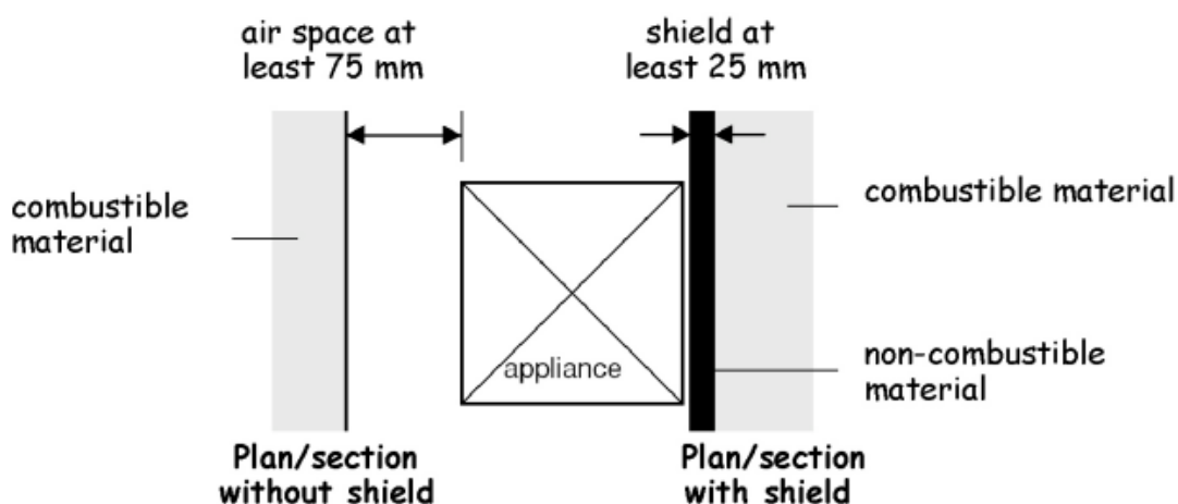
Figure 3.52 Plan of appliance on a hearth (separation)
