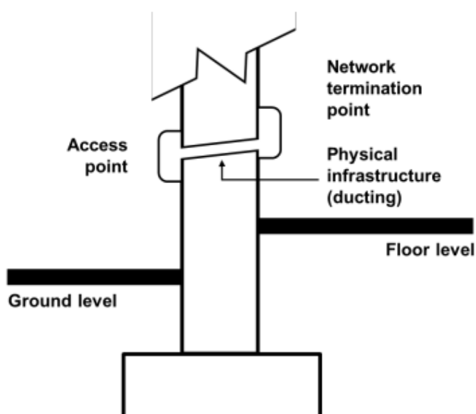
Figure 4.12 In-building physical infrastructure serving a single occupancy building
