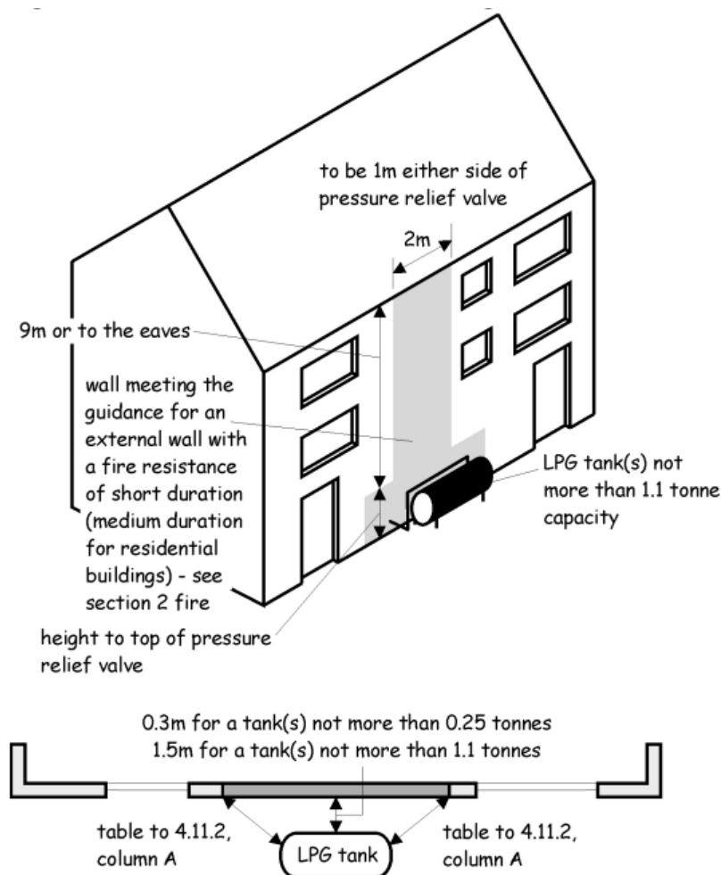
Figure 4.11 Small LPG tank close to a building
