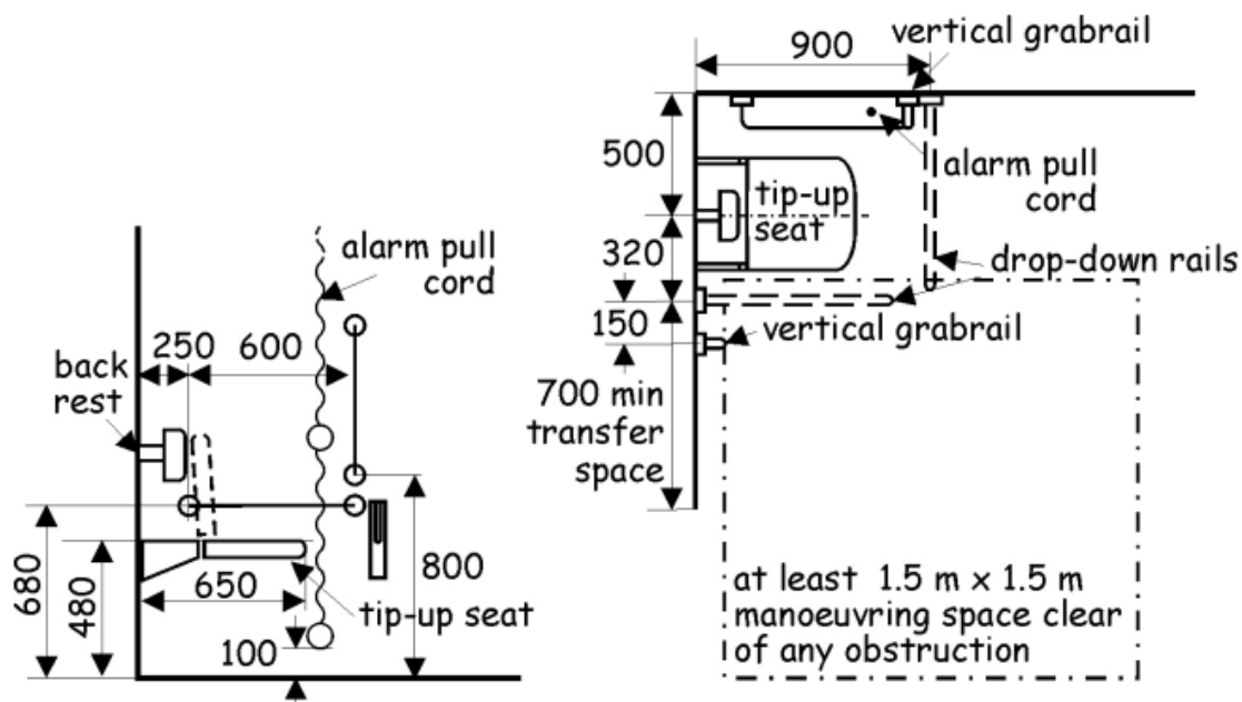
Figure 3.40 Example of Changing Places Toilet layout
