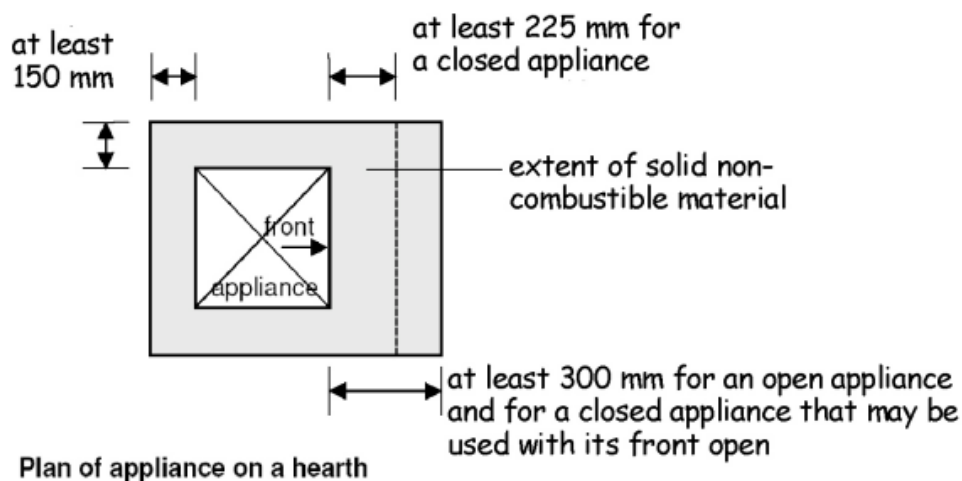
Figure 3.48 Appliance location
