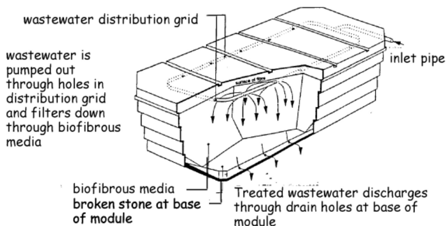
Figure 3.16 Typical proprietary filtration system
