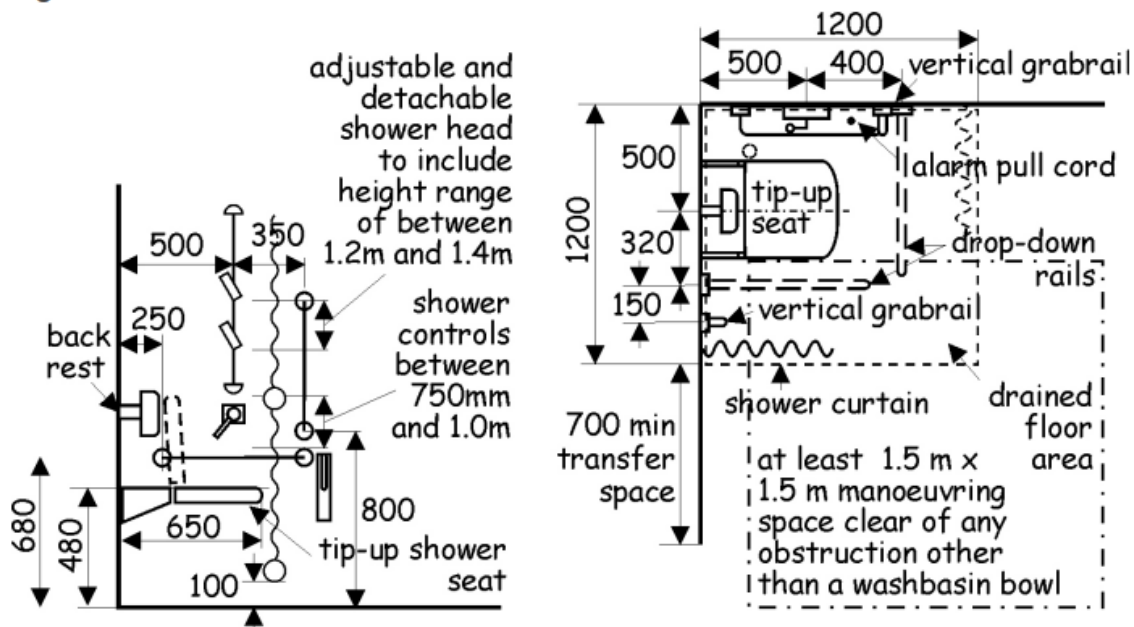
Figure 3.38 Provisions within an accessible shower room
