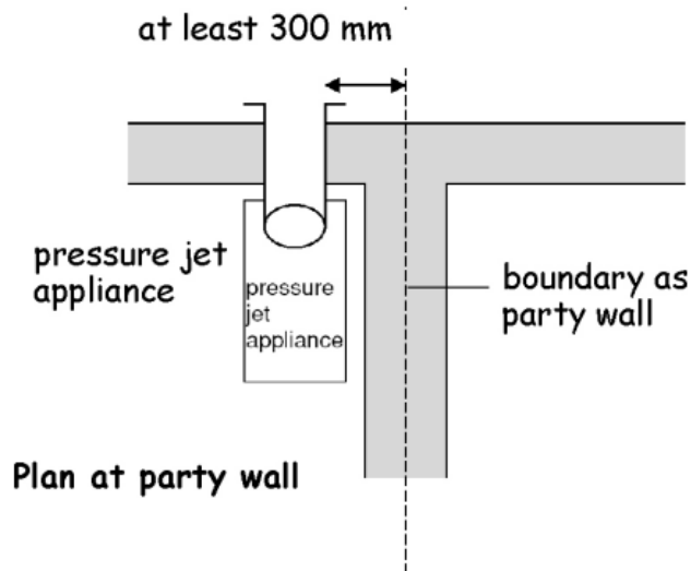
Figure 3.61 Separation between a boundary and terminal at right angles
