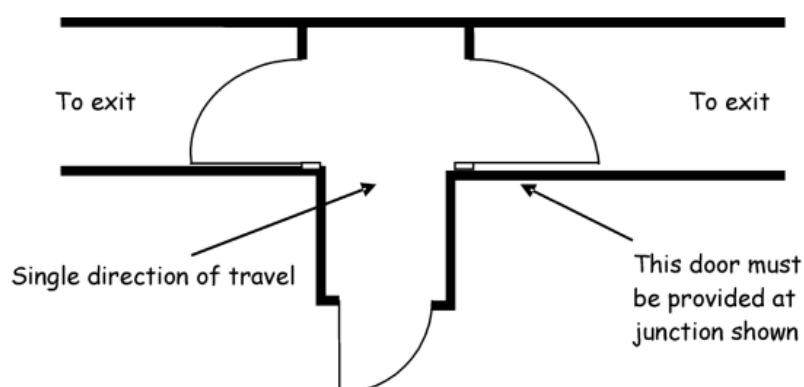
Figure 2.10 Corridor division
