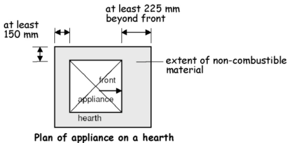
Figure 3.51 Plan of appliance on a hearth (gas-fired)
