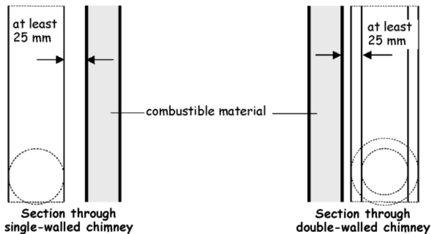
Figure 3.45 Section through double-walled chimney (horizontal)
