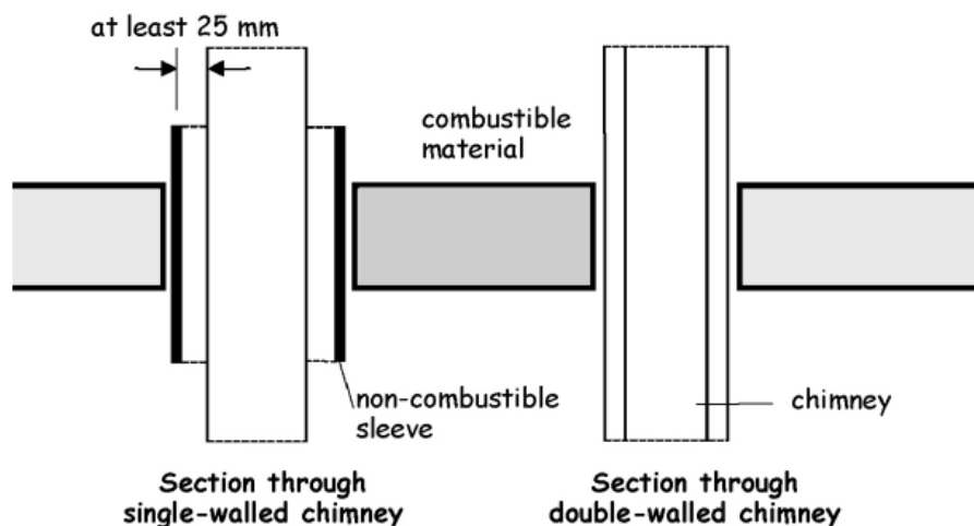
Figure 3.44 Section through single-walled chimney (vertical)
