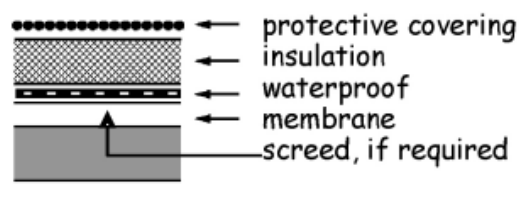
Figure 3.26 Roof constructions -Type B
