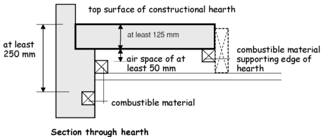
Figure 3.54 Section through hearth
