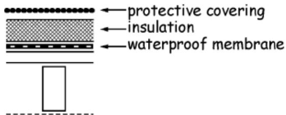
Figure 3.28 Roof constructions –Type D
