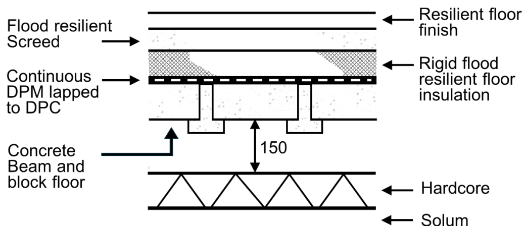
Figure 3.2 Suspended concrete floor
