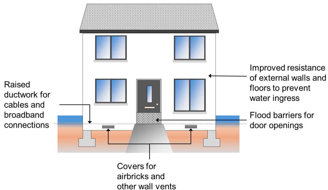
Figure 3.65: Resistance measures
