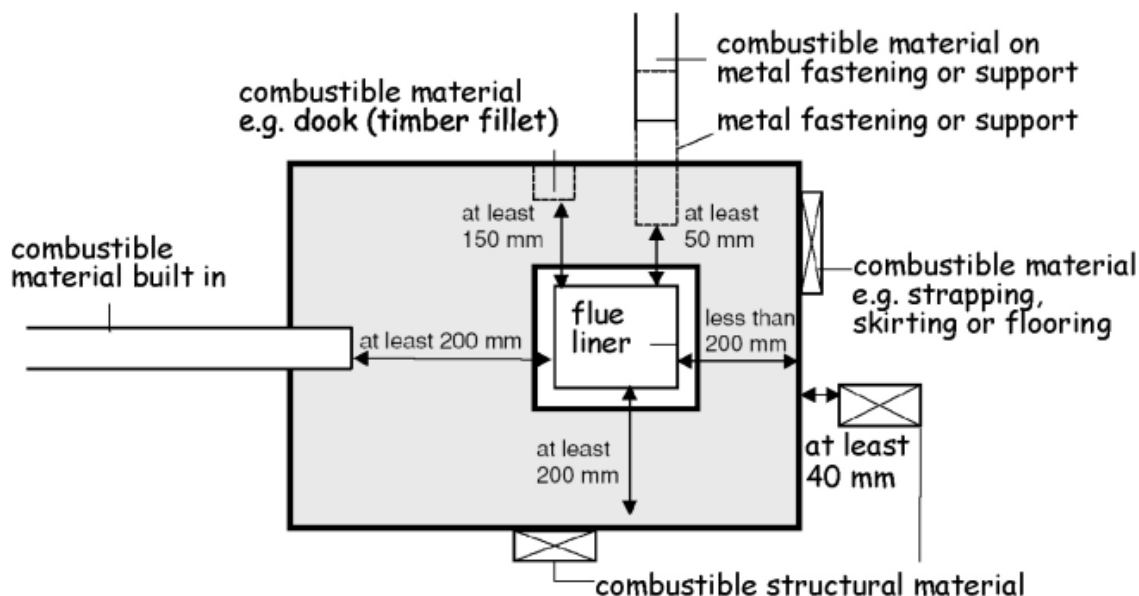
Figure 3.42 Plan view of masonry chimney
