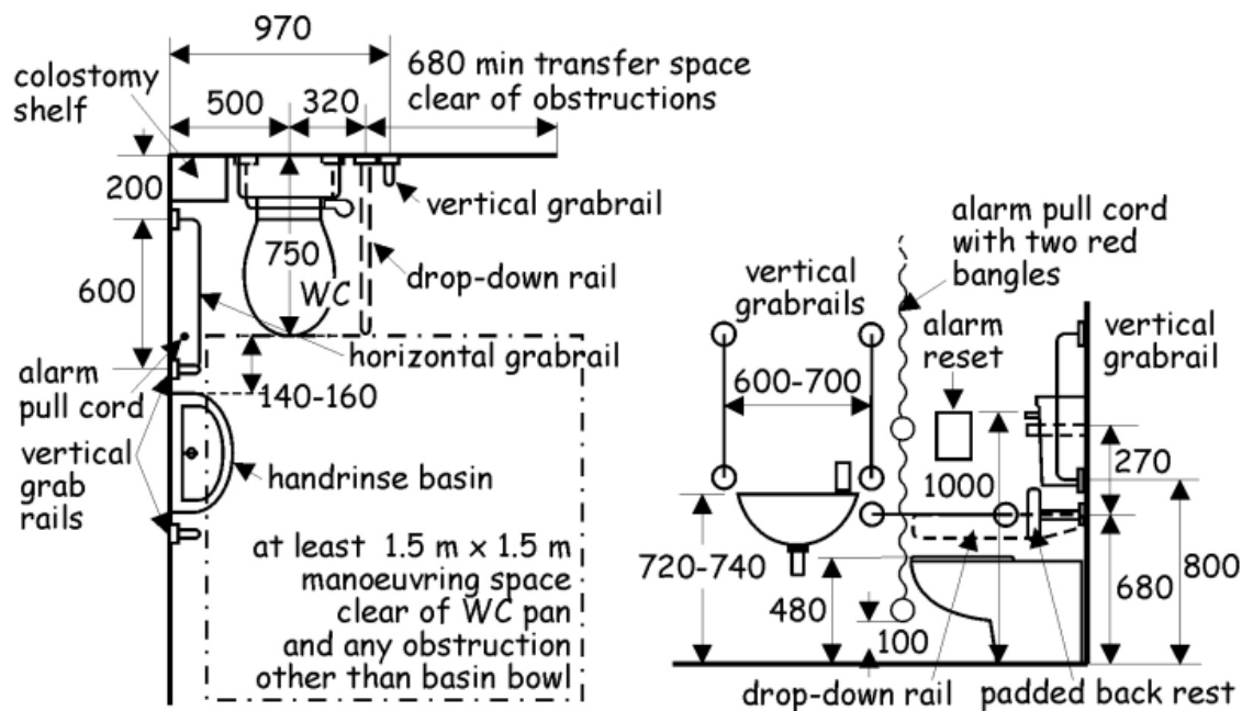
Figure 3.36 Provision within an accessible toilet
