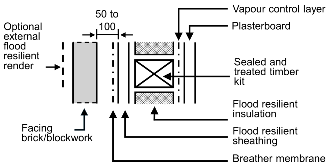
Figure 3.6 Wall construction – Timber framed and masonry cladding
