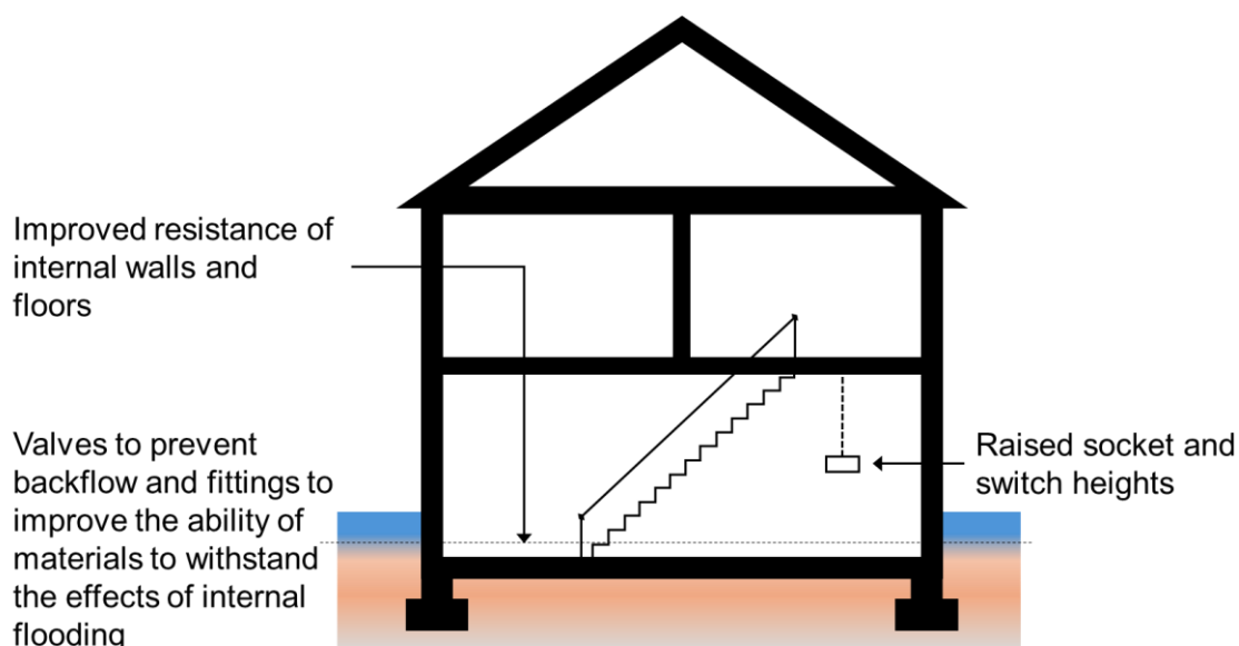
Figure 3.64: Recoverability measures
