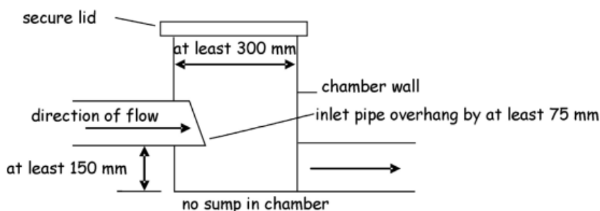
Figure 3.14 Section through inspection chamber
