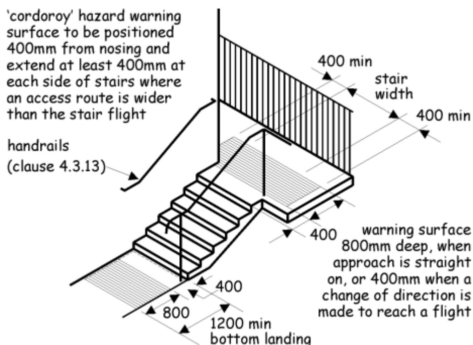
Figure 4.6 Use of corduroy tactile paving
