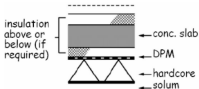
Figure 3.8 Ground supported concrete floors 2
