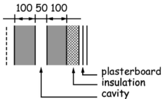
Figure 3.19 Wall constructions - Type A
