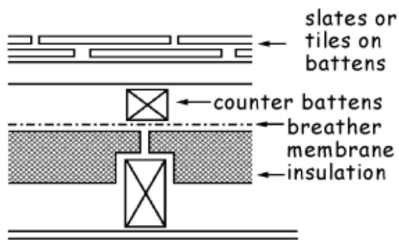
Figure 3.33 Roof constructions -Type C
