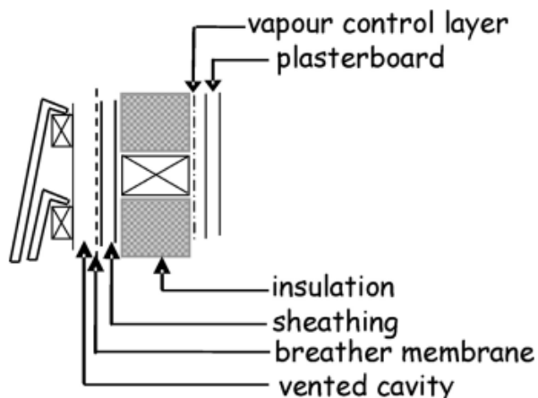
Figure 3.23. Wall constructions - Type B
