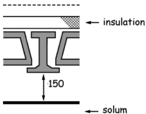
Figure 3.10 Suspended concrete Floors
