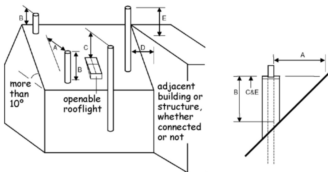
Figure 3.58 Solid fuel - flue outlets
