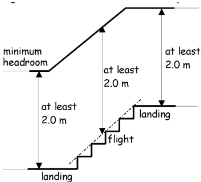
Figure 4.8 Headroom on stairs and ramps
